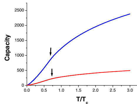
FIG. 1 (color online). The channel capacity, for the case of noninteracting bosons, plotted against T/T_c . The lower curve is for the case of 100 bosons, in a 3D box with PBC. For ^{87}\text{Rb} atoms in such a box of volume 1 \mu\text{m}^3 , thermodynamical calculations predict T_c \approx 0.4 \mu\text{K} . The upper curve is for 500 bosons in the same trap. The thermodynamical estimations of T_c are higher than the corresponding values that we obtain (as indicated by the arrows).
