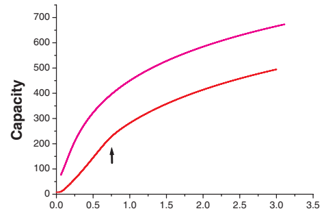
FIG. 2 (color online). We compare the channel capacity for the case of 100 (noninteracting) spinless fermions (upper curve) with that of 100 bosons (lower curve). The trap is a 3D box with PBC. For the lower curve, the horizontal axis is T/T_c , while for the upper curve, it is T/T_f , where T_f = (\hbar^2/2mk_B) \times (3\pi^2 N/gL^3)^{2/3} is the Fermi temperature.
