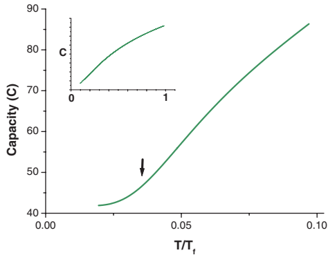
FIG. 3 (color online). Channel capacity of 100 interacting fermions in a 3D box trap with PBC, against T/T_f . The capacity is initially convex, and then becomes concave, for higher T 's, as illustrated in the inset.
